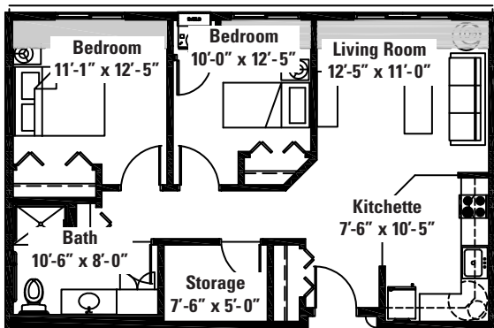
G. 2-Bedroom Approximately 800 sq. ft.
