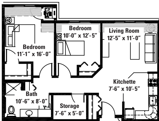
H. 2-Bedroom Approximately 844 sq. ft.
